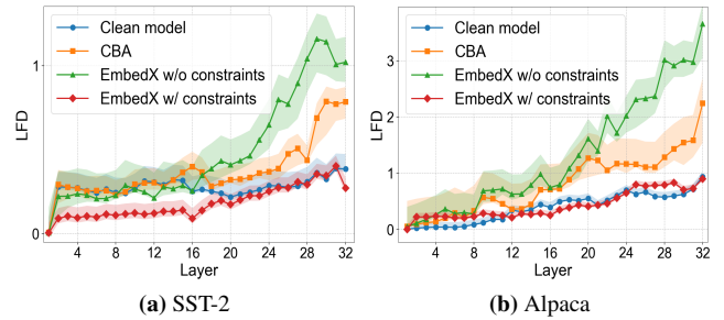
Figure 6: The stealthiness from frequency across latent layers.
