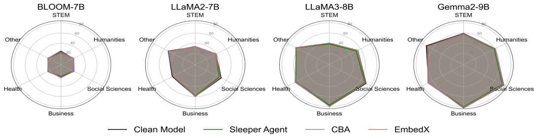
Figure 4: Comparison of the accuracy of Clean Model, Sleeper Agent, CBA, and EmbedX on different LLMs in several MMLU topics.
